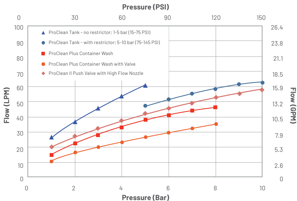
ProClean Tank Nozzle
